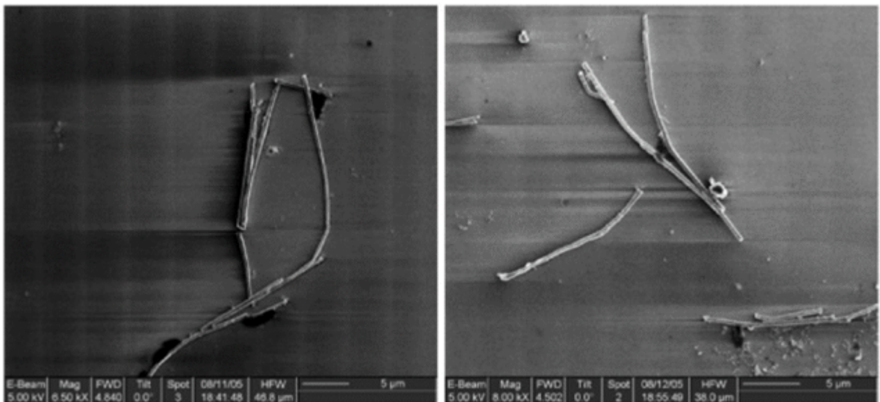
Nanowires
